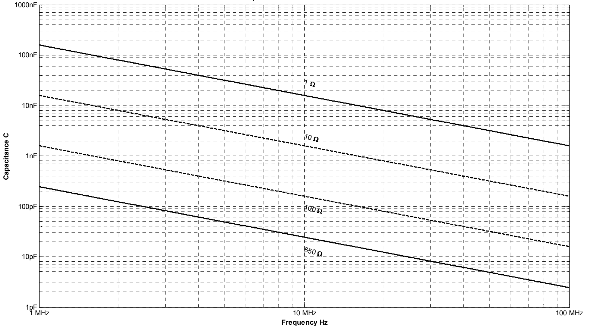
Capacitance Measurement MFJ259B
