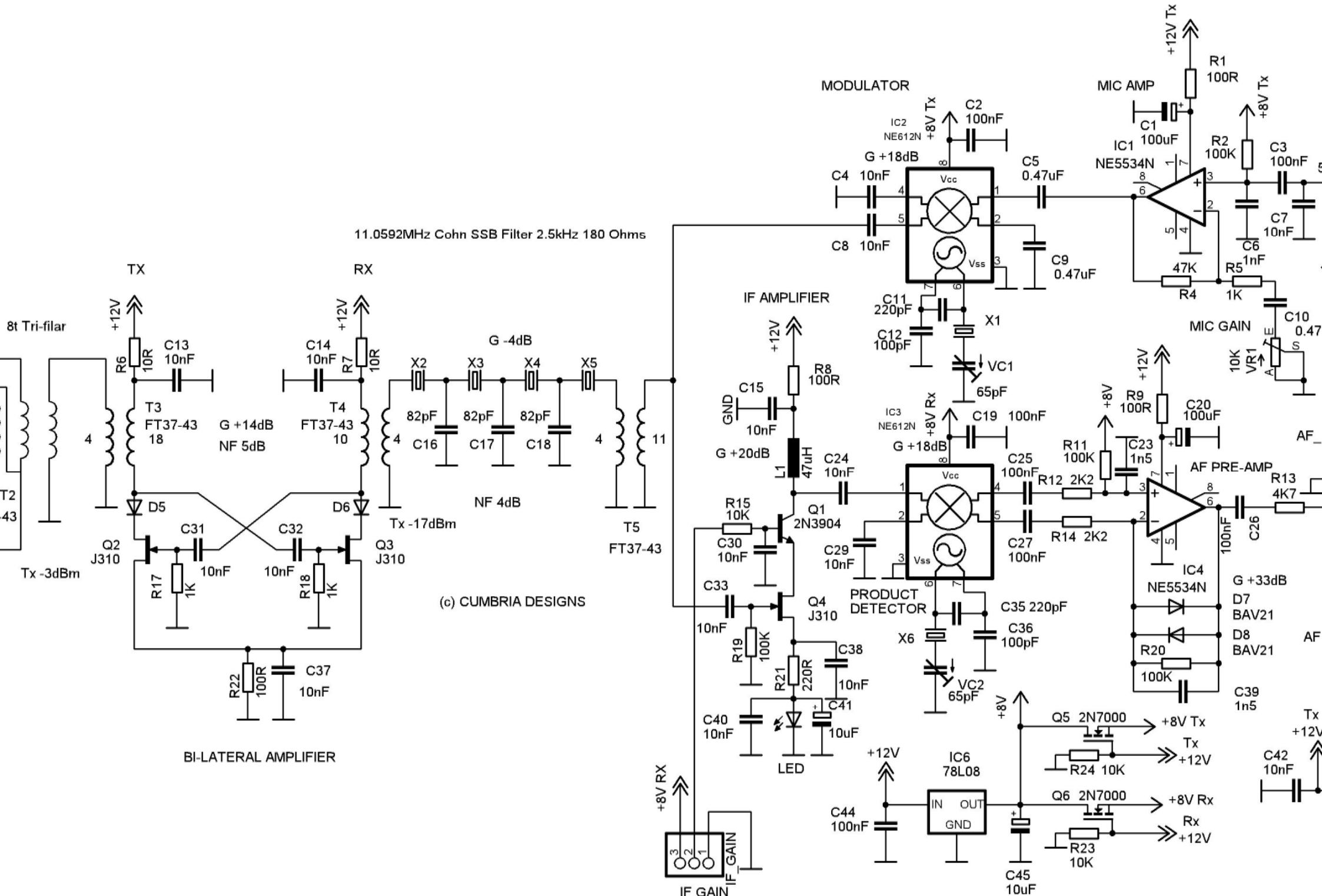
Eden SSB IF System Schematic
