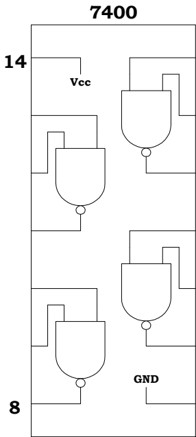
QUAD NAND
