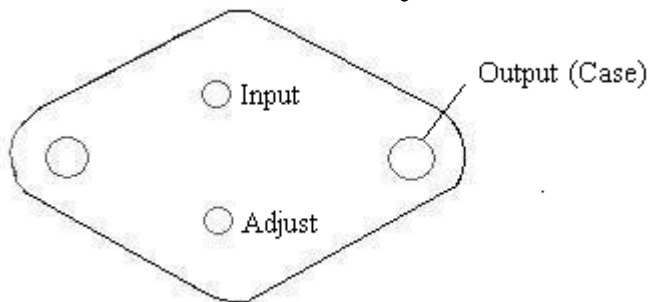
Underside View
