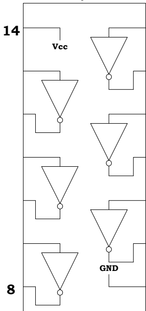
HEX INVERTER
