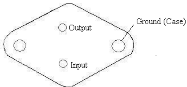
Underside View
