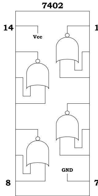
QUAD NOR
