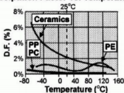
Dissipation Factor vs. Temperature
