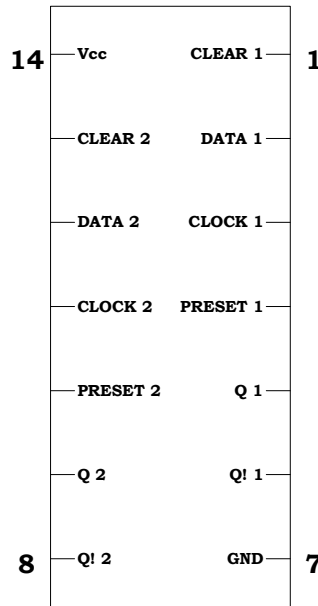
DUAL D FLIP-FLOP
