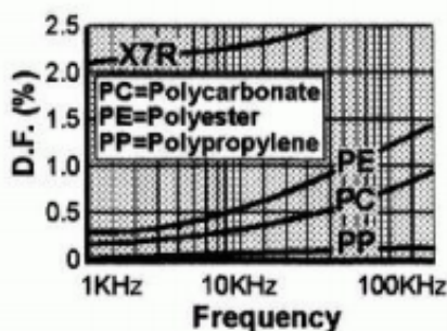
Dissipation Factor vs. Frequency
